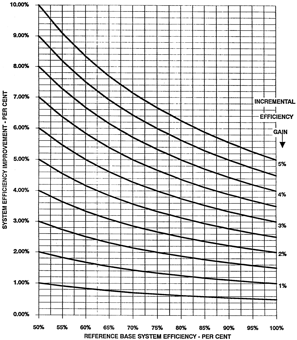
Figure I1-5. System Efficiency Improvement as a Function of Incremental Component Efficiency Gain
