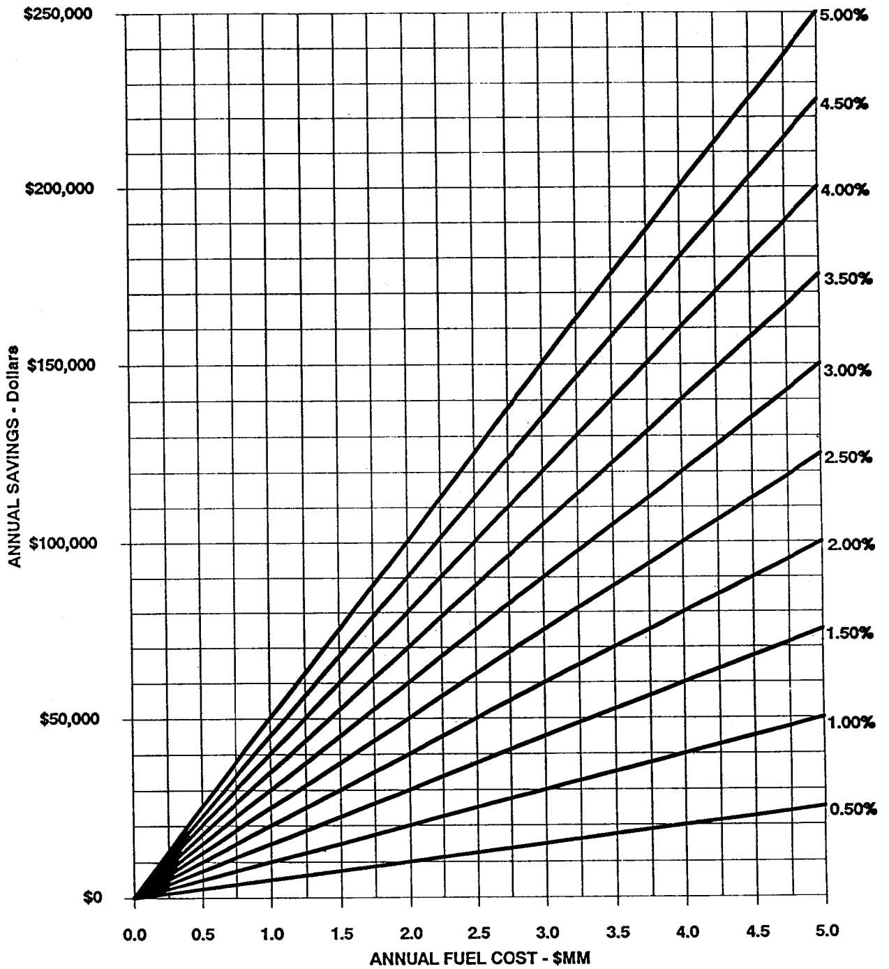
Figure I1-6. Annual Savings as a Function of Annual Fuel Cost and System Efficiency Improvement
