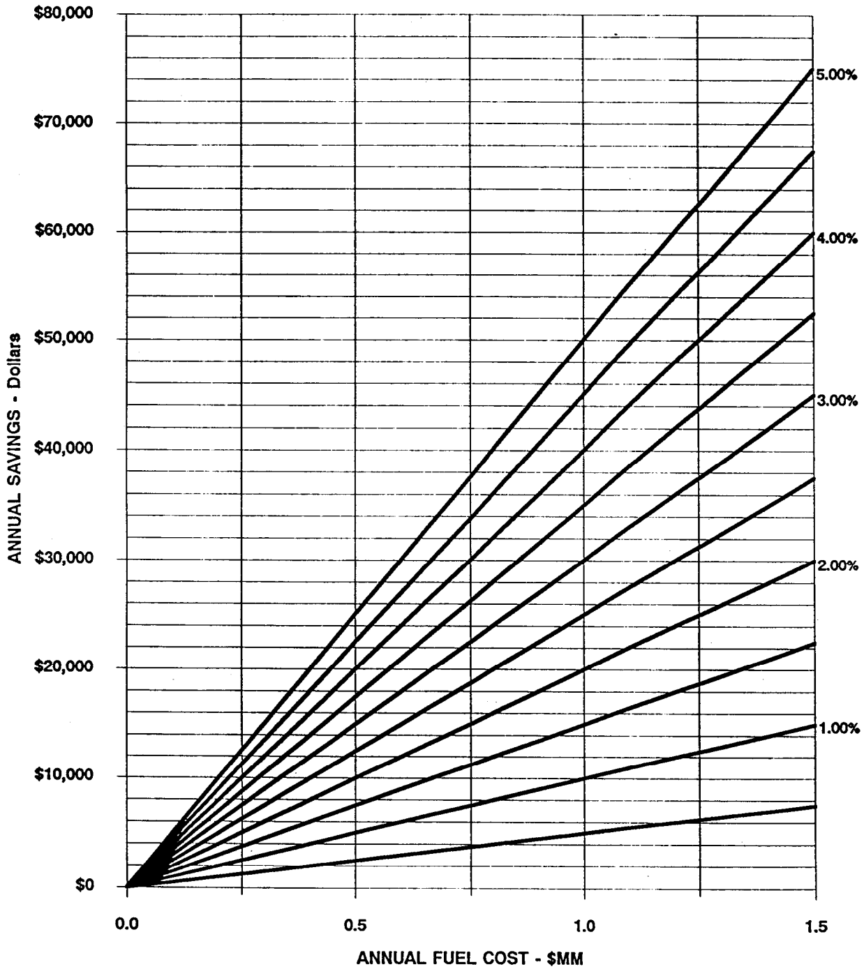
Figure I1-7. Annual Savings as a Function of Annual Fuel Cost and System Efficiency Improvement (Expansion of Figure I1-6)
